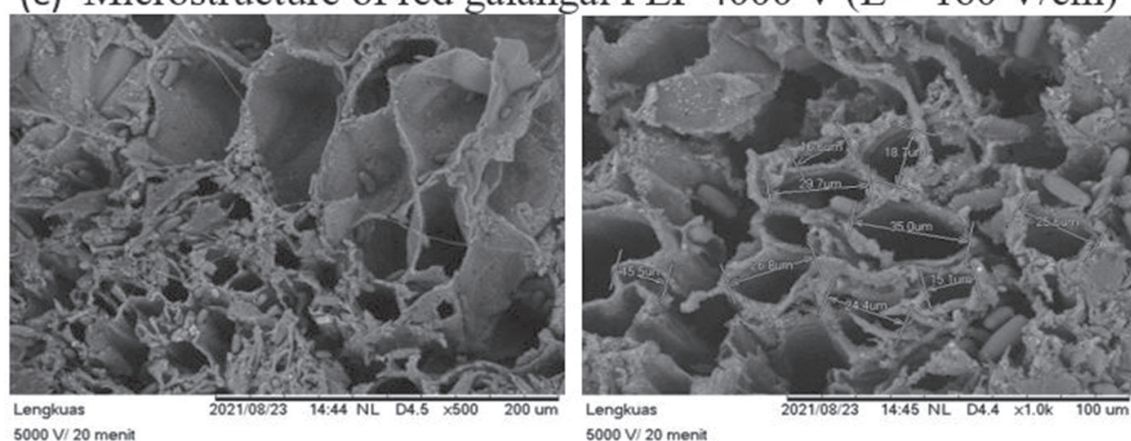
Fig. 3. The microstructure of galangal rhizome
